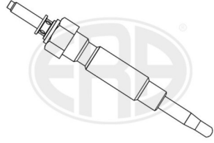
VELA AQUEC. MOTOR NISSAN 110654P400 =CP04
