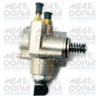
BOMBA ALTA PRESSAO VAG 1.4TSI 03C127025T GOLF V = 133062+b
