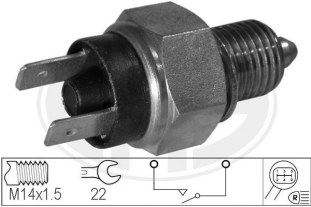
INTERRUPTOR LUZ M/A FIAT 4143288 ALFA = 40500+c
