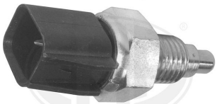
INTERRUPTOR LUZ M/A OPEL 4803447 =40506 =36140 0912097
