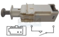
INTERRUPTOR LUZ STOP FIAT 2F 51798630 =24791
