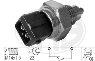
INTERRUPTOR LUZ M/A PSA 96018108 PARTNER =40650+c
