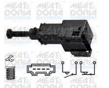
INTERRUPTOR LUZ STOP VAG 1J0945511 =330503 =24760
