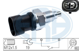
INTERRUPTOR LUZ M/A OPEL 1239266 =40510 =40830+c=36017 =36050
