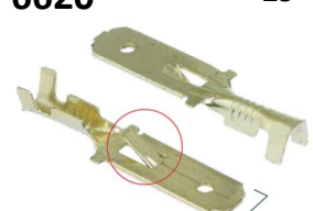
TERMINAL MACHO 6.3mm 0.5-1mm
