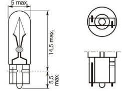
LAMPADA 12V 2,3W S/CASQUILHO W2x4.6d =17073
