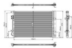
CONDENSADOR AC KIA 97606C8000 667484 CCSHY057
