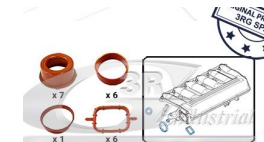
KIT JUNTAS COLETOR ADMISSAO BMW 11612246942 =BKSBM012B 85130RG
