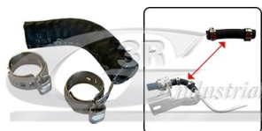
KIT TUBO VALVULA EGR RENAULT 223214742R TRAFIC III 1.6
