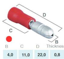
TERMINAL ISOLADO REDONDO =1864000 =190021 =RO400
