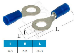
TERMINAL ISOLADO OLHAL AZUL 8781353125 =1857100 =190029 =817
