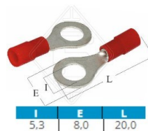
TERMINAL ISOLADO OLHAL 8781353122 =1853150 =190031 =719
