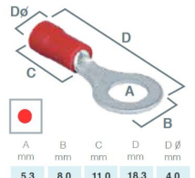
TERMINAL ISOLADO OLHAL =1853150 =190031 =RON053
