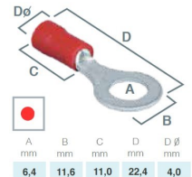
TERMINAL ISOLADO OLHAL P/FIO =1853200 =190015 =RON064
