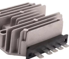
REGULADOR 12V JOHN DEERE AM101406
