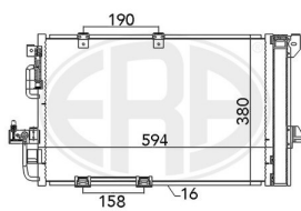
CONDENSADOR AC OPEL 09130610 =260010 =667043
