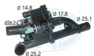
TERMOSTATO '83 PSA/FORD 1336AF =4006060 =92555
